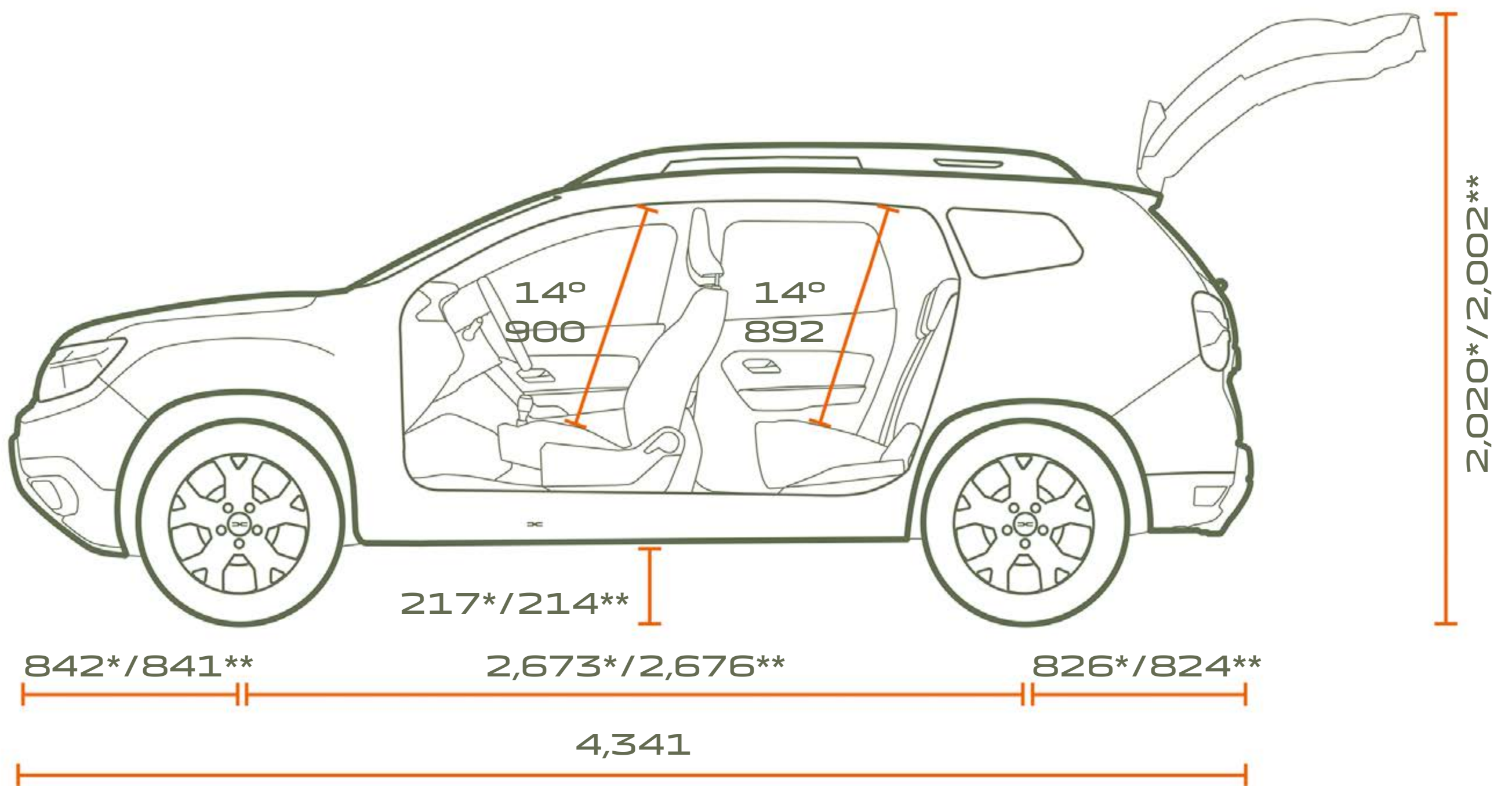
PROFILE VIEW
